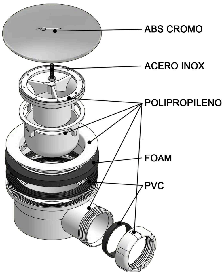
DESPIECE
